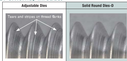
External threads cut by Solid Round Dies-D have less tears and stripes on thread flank face.
