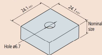
Rectangular gauge blocks
