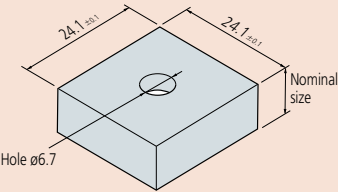
Square gauge blocks
