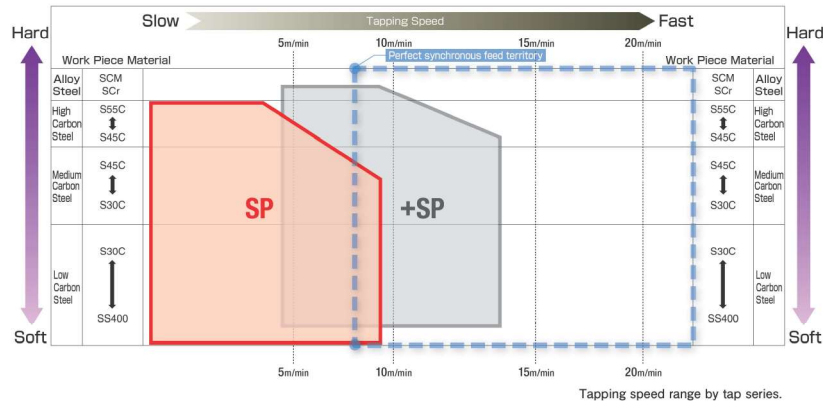
Tapping speed range by tap series.
