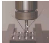
Chip evacuation with a SP tap.
